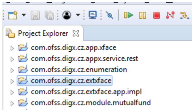
Figure 2 Project structure
