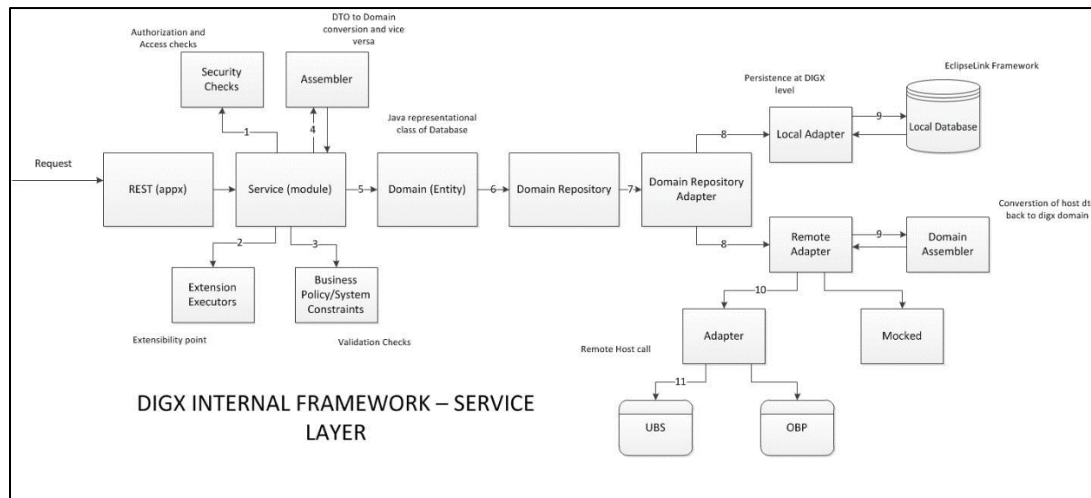
Figure 1 DIGX Service Layer
